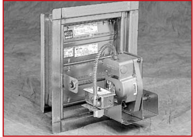
Fire/Smoke Damper with Factory Mounted Actuator and PFMA
