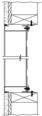
WOOD INSTALLATION
