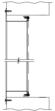
FLANGE MOUNT
