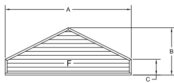
House (F)
