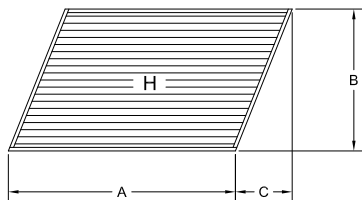
Parallelogram (H)
