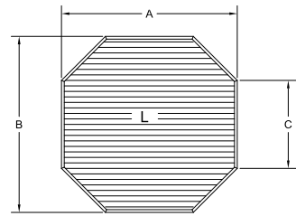
Octagon (L)
