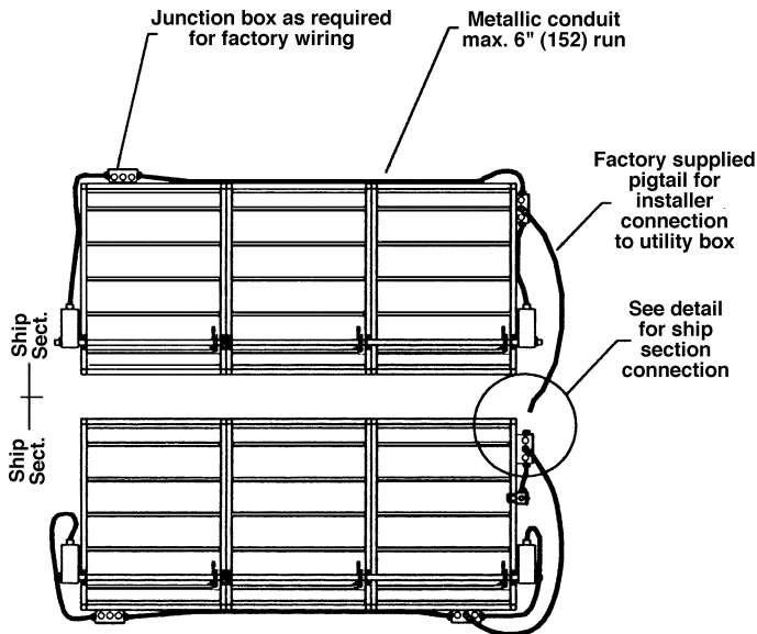
TYPICAL SHIP SECTION DETAIL
