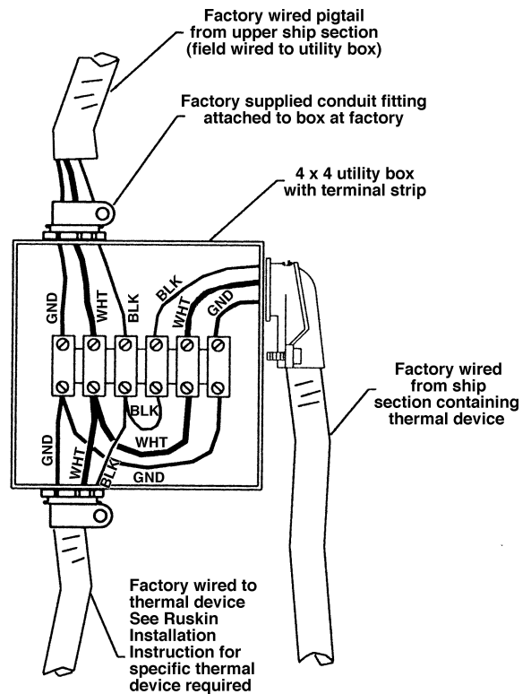
SHIP SECTION FIELD CONNECTION
