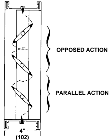
OPPOSED/PARALLEL BLADES
