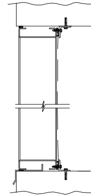
MASONARY WALL
