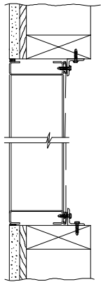
WOOD INSTALLATION
