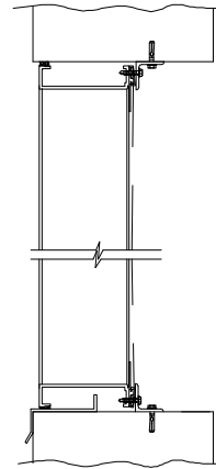
MASONRY WALL
