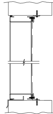
MASONARY WALL
