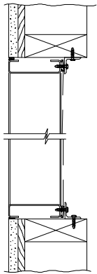
WOOD INSTALLATION
