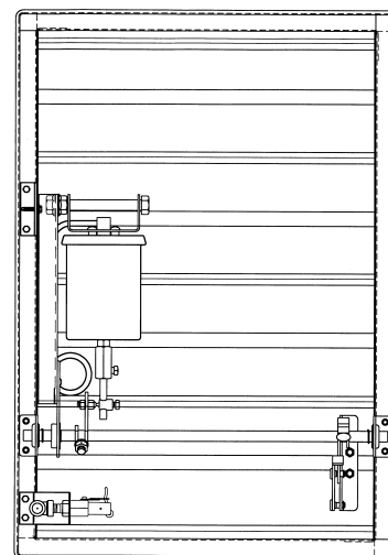
FSD shown with pneumatic actuator in airstream
