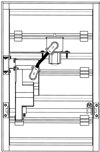
FSD shown with electric actuator in airstream
