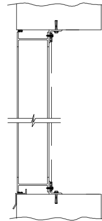
MASONARY WALL
