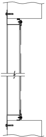
FLANGE MOUNT
