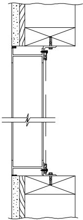
WOOD INSTALLATION
