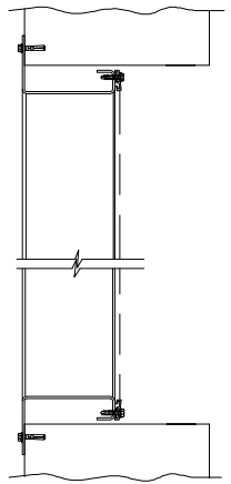
FLANGE MOUNT
