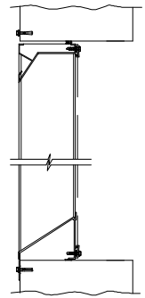
FLANGE MOUNT
