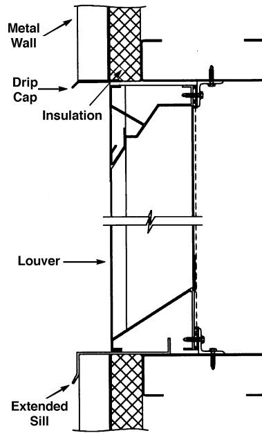
Flange Mount
