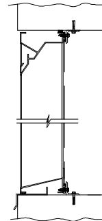
MASONARY WALL
