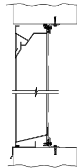
MASONARY WALL
