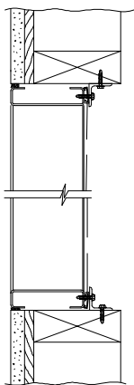
WOOD INSTALLATION
