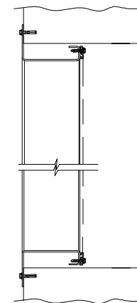
FLANGE MOUNT
