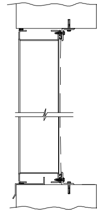
MASONRY WALL
