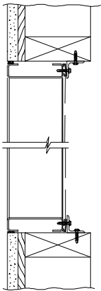
WOOD INSTALLATION
