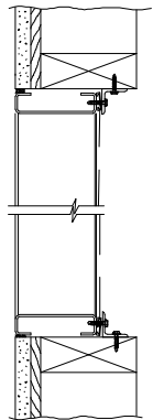
WOOD INSTALLATION
