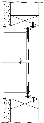
WOOD INSTALLATION
