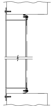
FLANGE MOUNT
