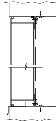
MASONRY WALL
