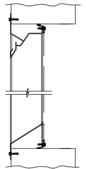
FLANGE MOUNT
