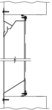
FLANGE MOUNT
