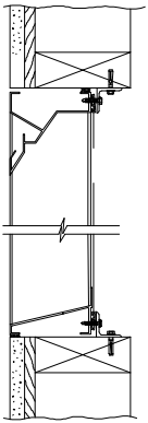
WOOD INSTALLATION
