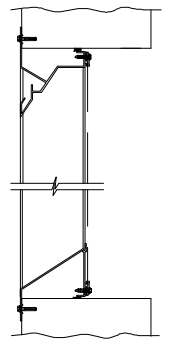
FLANGE MOUNT
