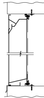
MASONRY WALL
