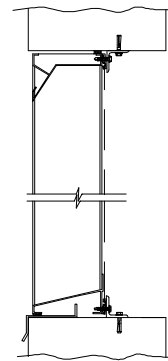
MASONRY WALL
