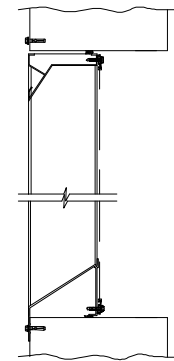
FLANGE MOUNT
