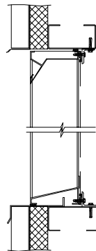
METAL PANEL WALL
