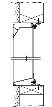
WOOD INSTALLATION
