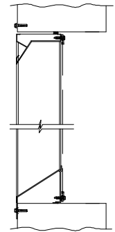
FLANGE MOUNT
