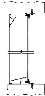
MASONRY WALL
