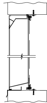
MASONARY WALL
