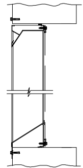
FLANGE MOUNT
