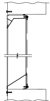
FLANGE MOUNT
