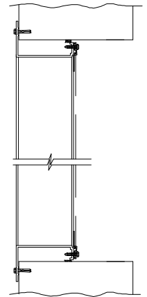
FLANGE MOUNT
