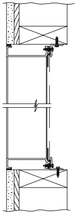
WOOD INSTALLATION
