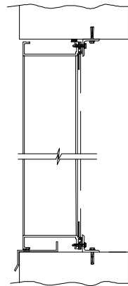
MASONRY WALL
