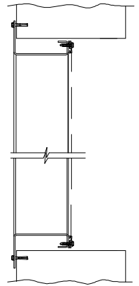
FLANGE MOUNT
