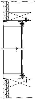
WOOD INSTALLATION
