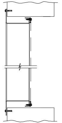
FLANGE MOUNT
