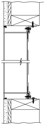
WOOD INSTALLATION
