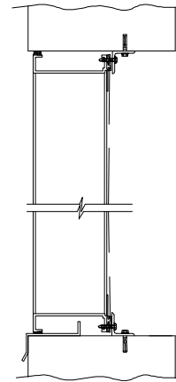
MASONARY WALL
