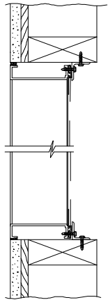
WOOD INSTALLATION
