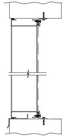
MASONARY WALL
