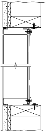
WOOD INSTALLATION
