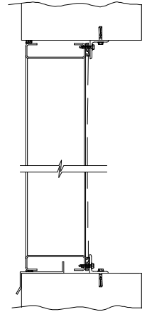
MASONRY WALL
