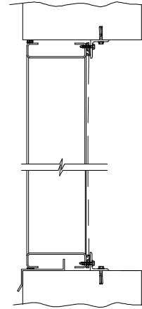
MASONRY WALL
