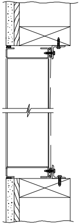
WOOD INSTALLATION
