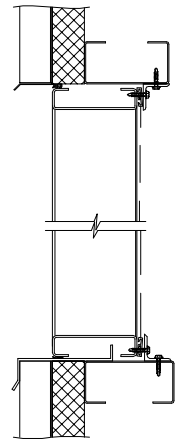
METAL PANEL WALL
