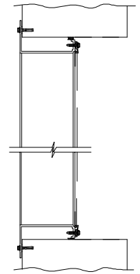
FLANGE MOUNT
