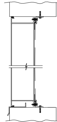
MASONARY WALL
