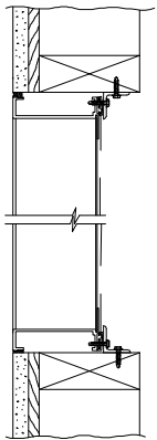
WOOD INSTALLATION
