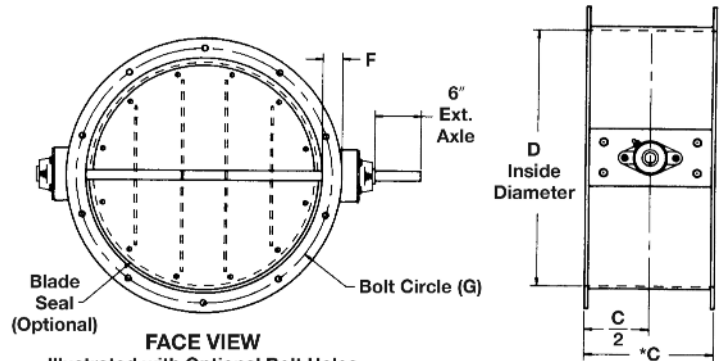
Illustrated with Optional Bolt Holes
