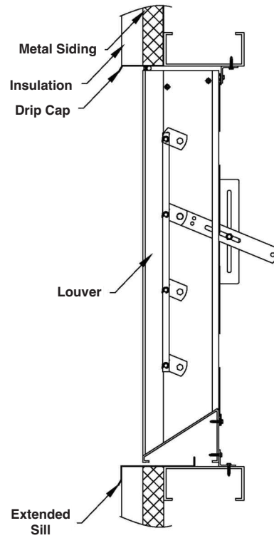
Flange Mount
