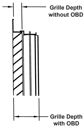
GRILLE DETAIL
