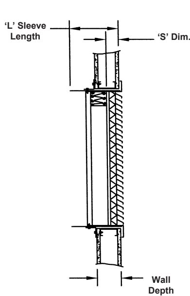
DUCTED
