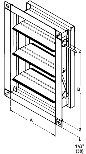
SINGLE SECTION DAMPER WITH FLANGE FRAME OPTION
