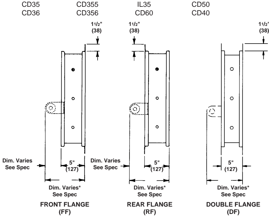
SINGLE SECTION DAMPER WITH FLANGE FRAME OPTION
