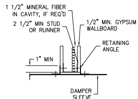
1 HR WALL RATING
