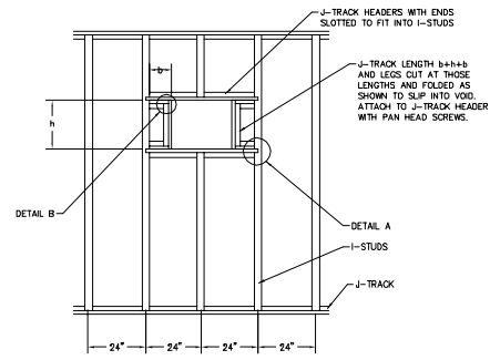
FRAMING DETAIL U497
