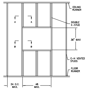
FRAMING DETAIL U438
