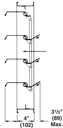
VERTICAL MOUNT HORIZONTAL AIR FLOW
