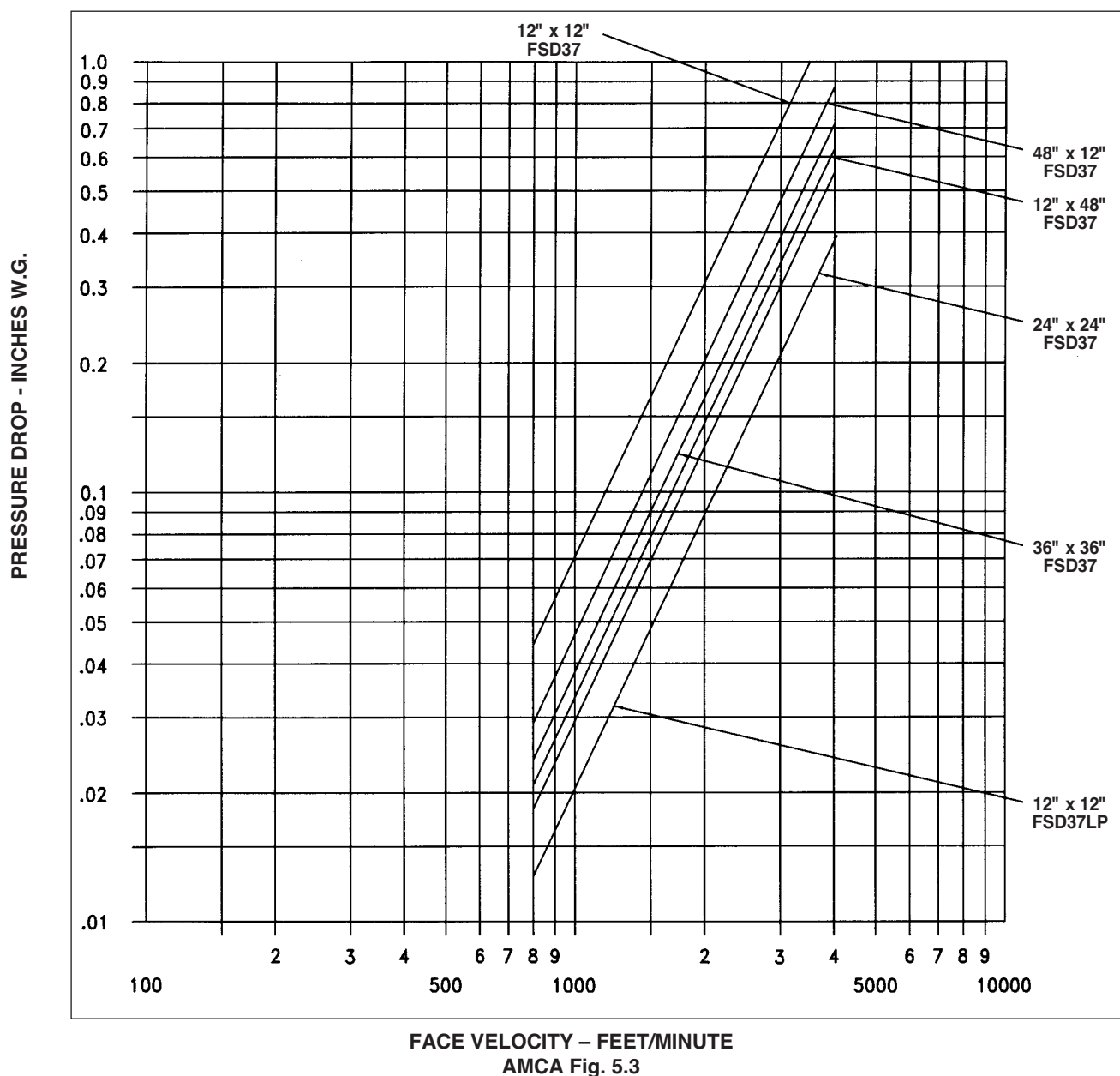
VELOCITY vs. PRESSURE DROP
