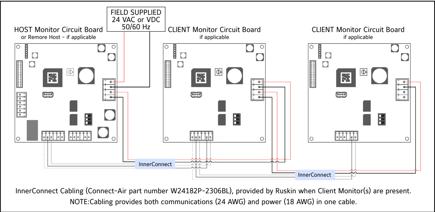
Typical Wiring Configuration
