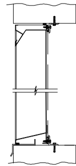
MASONRY WALL
