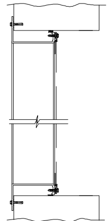
FLANGE MOUNT
