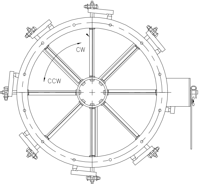
VIEW FROM AIR INLET SIDE INLET AIR ROTATION (CW OR CCW) DETERMINED FROM AIR INLET SIDE OF FAN
