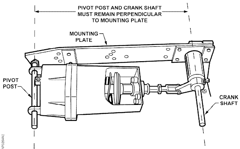
Figure 7. Perpendicular Mounting.
